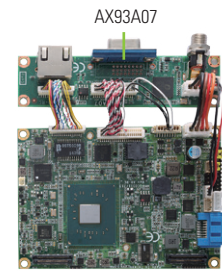
▲ Assembly view
