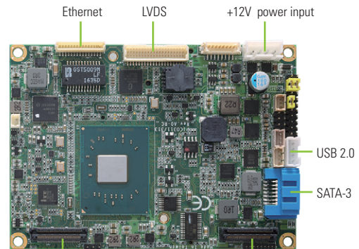
4 x USB 3.0, 1 x PCIe x1, DDI HD audio, LPC, power on/off, reset, LED
